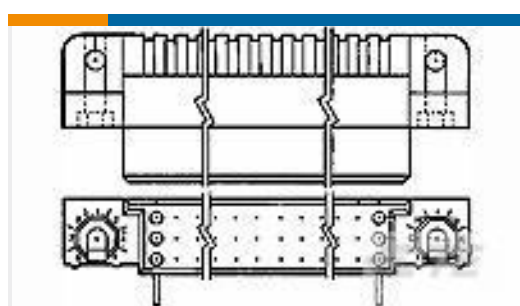
TE 零件编号103741-1 01 MODII HDR SRST B/A . 100CL
